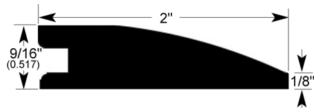
STANDARD REDUCER
