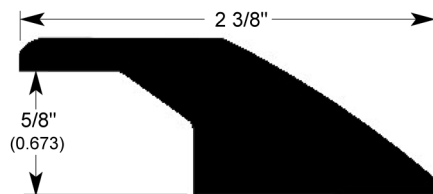
OVERLAP REDUCER
