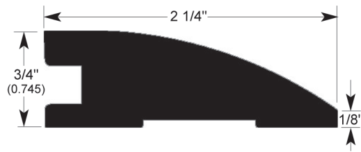
STANDARD REDUCER
